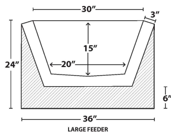
LARGE FEEDER
