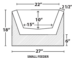
SMALL FEEDER
