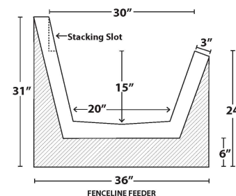
FENCELINE FEEDER
